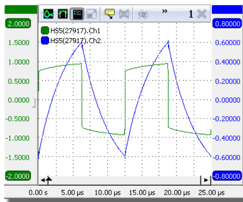
Figure 2.3: Yt graph.
