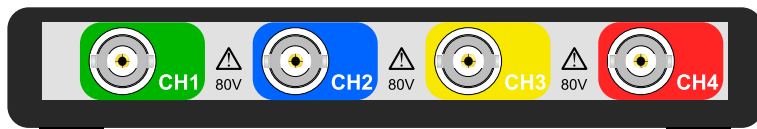
Figure 7.1: Front panel
