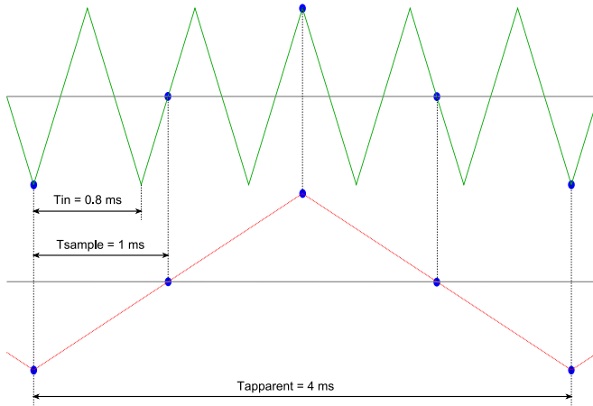
Figure 3.4: Aliasing
