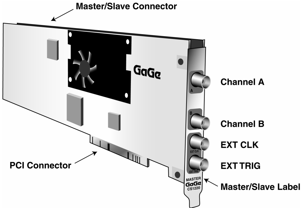
Figure 1: Connectors on CS1220
