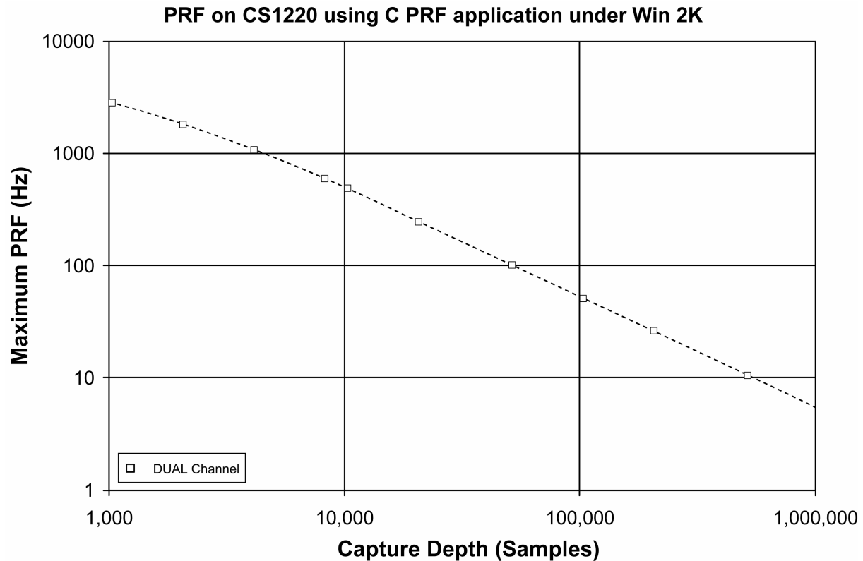
Figure 2: Maximum PRF vs. acquisition length
