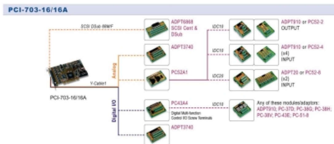
Figure 3-A PCI 703 Interconnections
