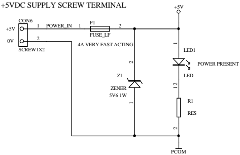
EXTERNAL +5VDC SUPPLY SCREW TERMINAL
