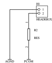
AGND TO POWER COMMON JUMPER
