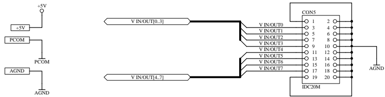
(8X) ANALOG INPUT/OUTPUTS (20WAY RIBBON CABLE)
