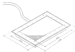
Extraction Table
