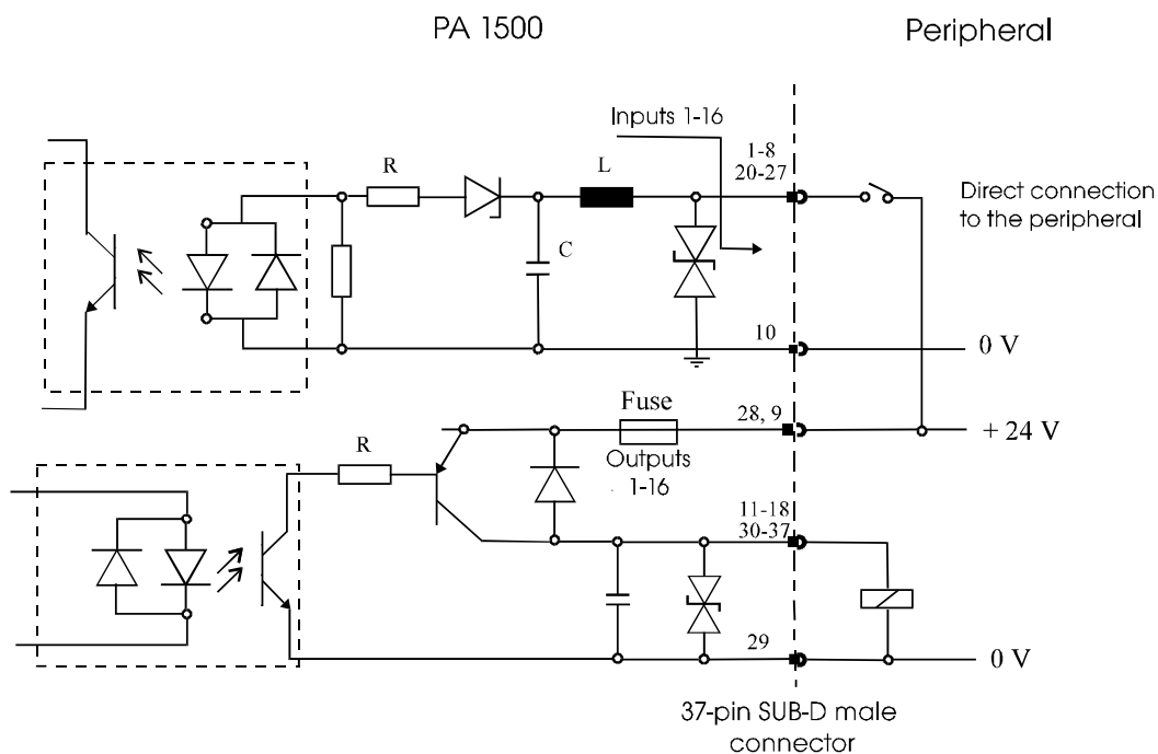
Fig. 8-2: Connection principle
