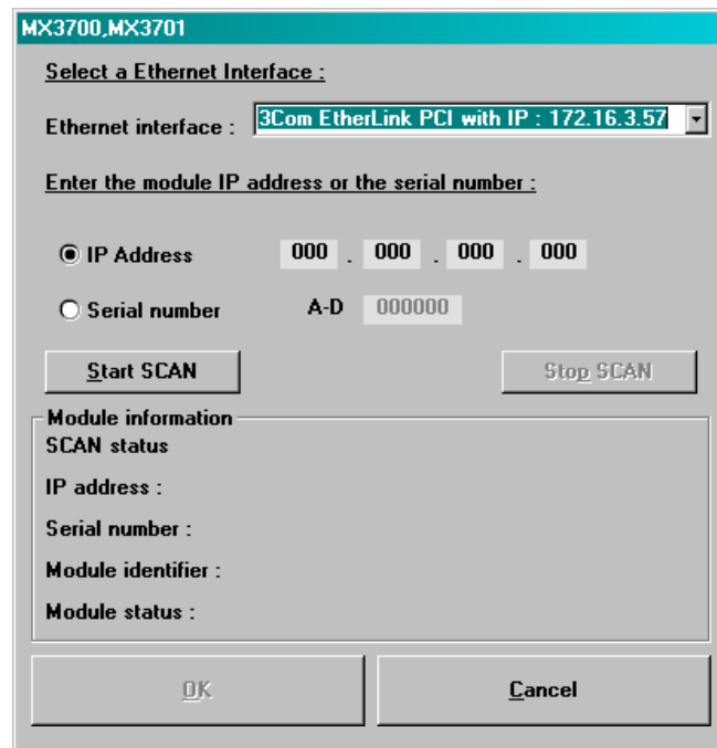
Fig. 7-3: Settings
