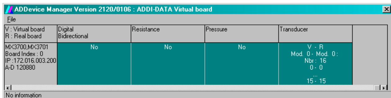
Fig. 7-7: ADDevice Manager
